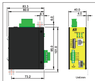
KSC-361-S4 Panel & Wall Mount Dimension
