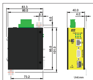
KSC-361-S2 Panel & Wall Mount Dimension
